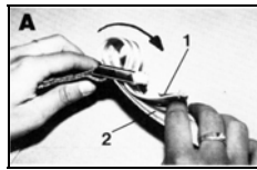
Figure A: Fold the strap to a loop and insert it upwards throughout the metal frame and turn the loop as indicated.
